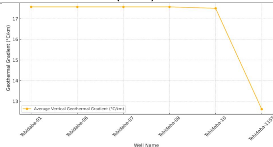
Fig. 3: Line Chart of Geothermal Gradient by Well
