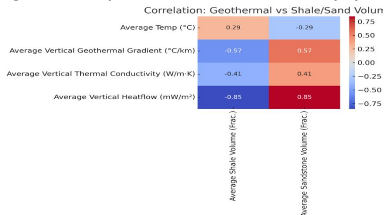
Fig. 6: Heatmap of All Geothermal and Petrophysical Correlations
