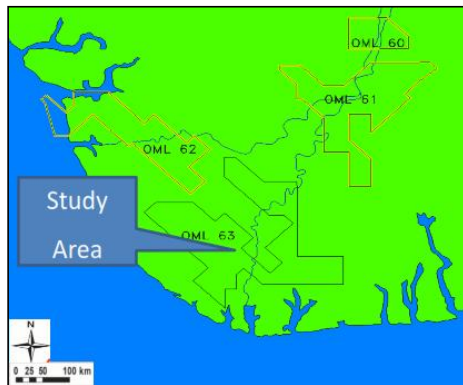
Figure 1: Map of Niger Delta showing Benin, the study Area (Doust and Omatols (1990) and
